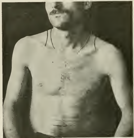
FIG. 258.—Krönig's isthmus. Both sides narrow due to bilateral tuberculosis.
